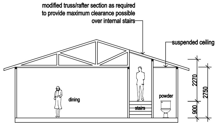
TRUSS SECTION T-T
