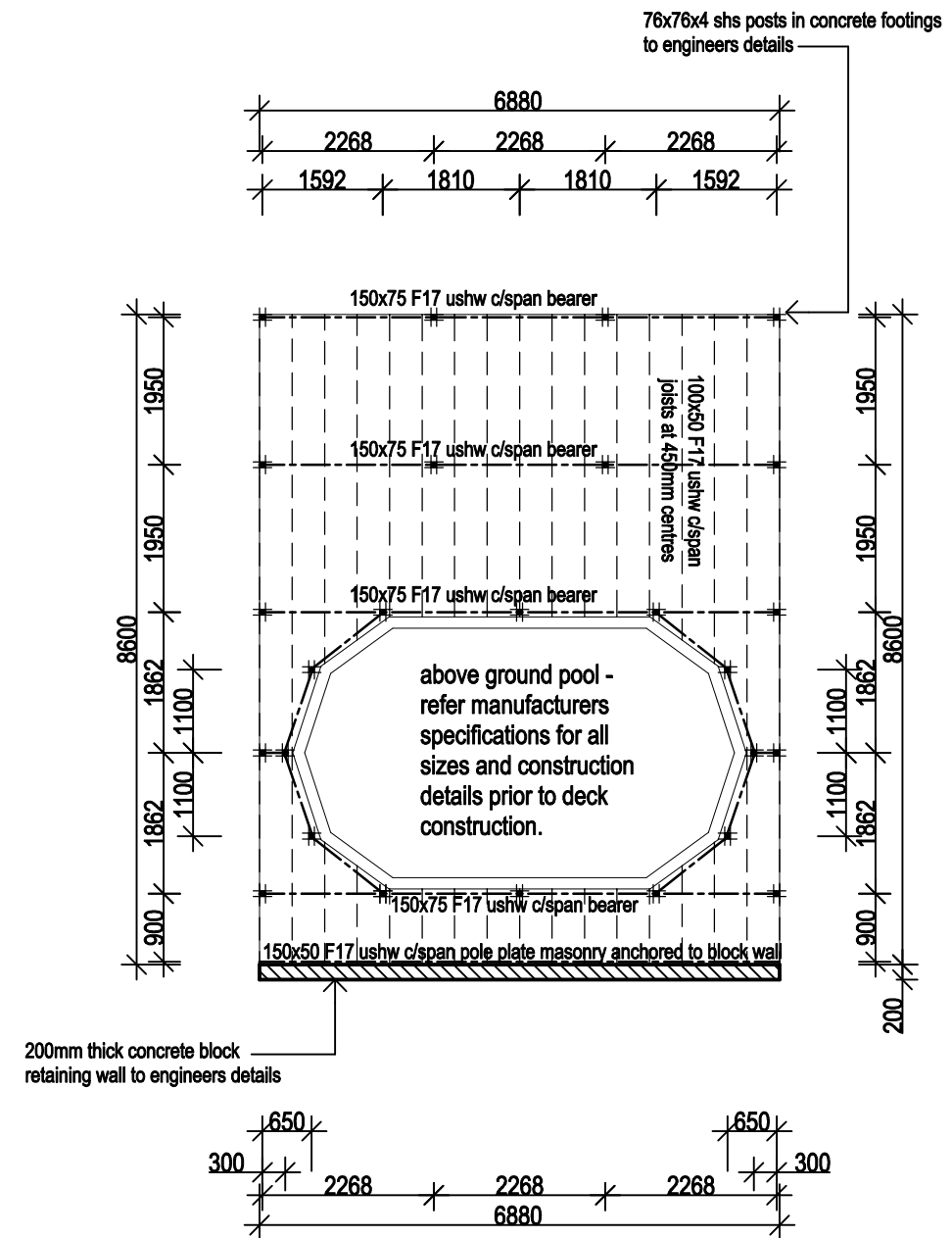
POOL DECK FRAMING PLAN
