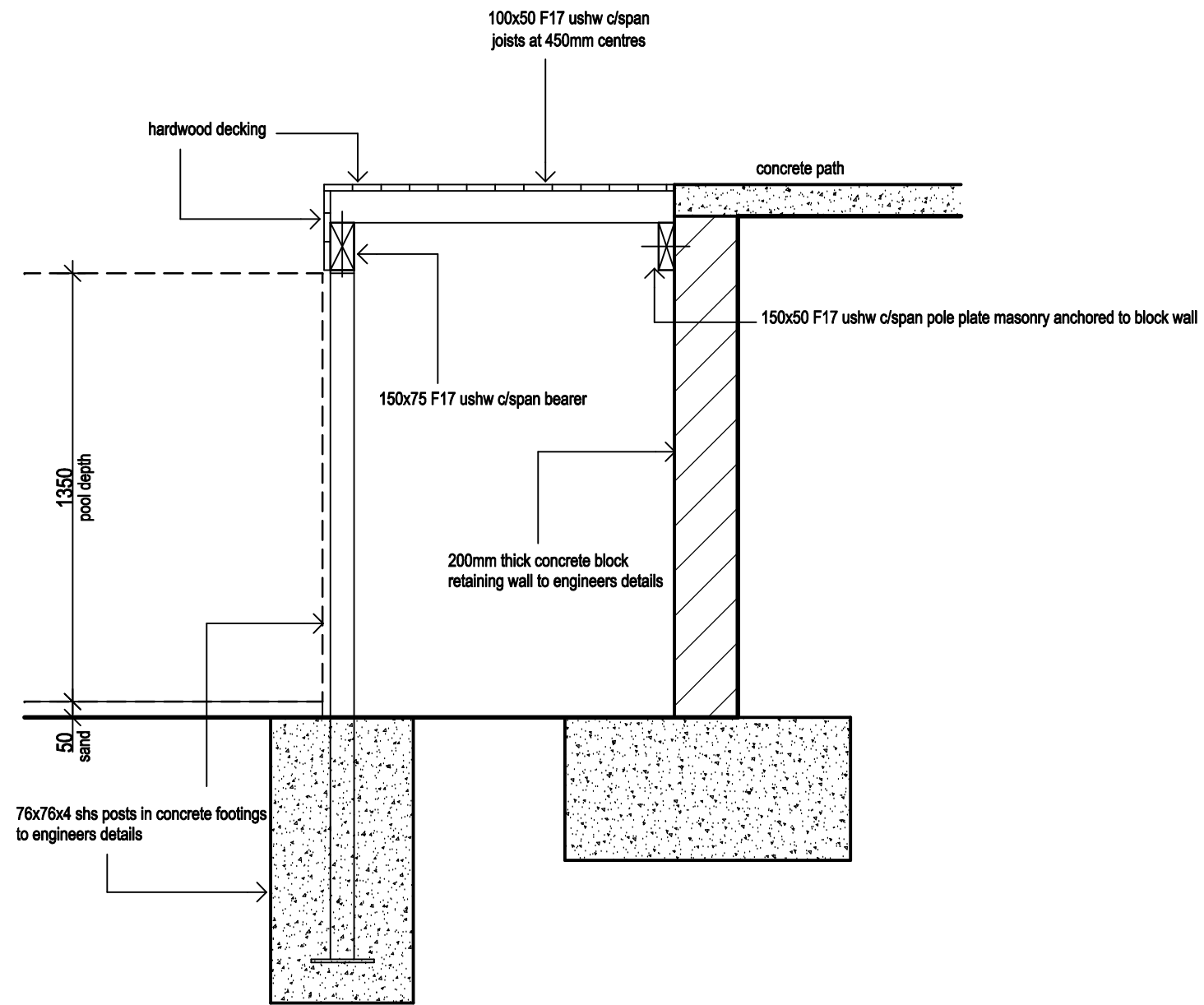
POOL DECK DETAIL 1:20
