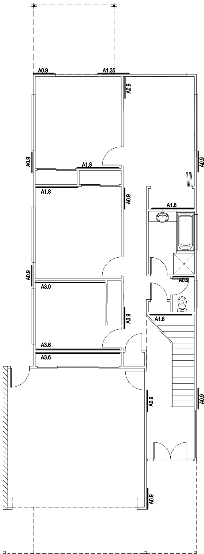
GROUND FLOOR
