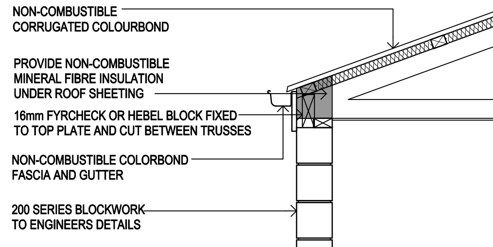
FIRE WALL DETAIL 1:20
