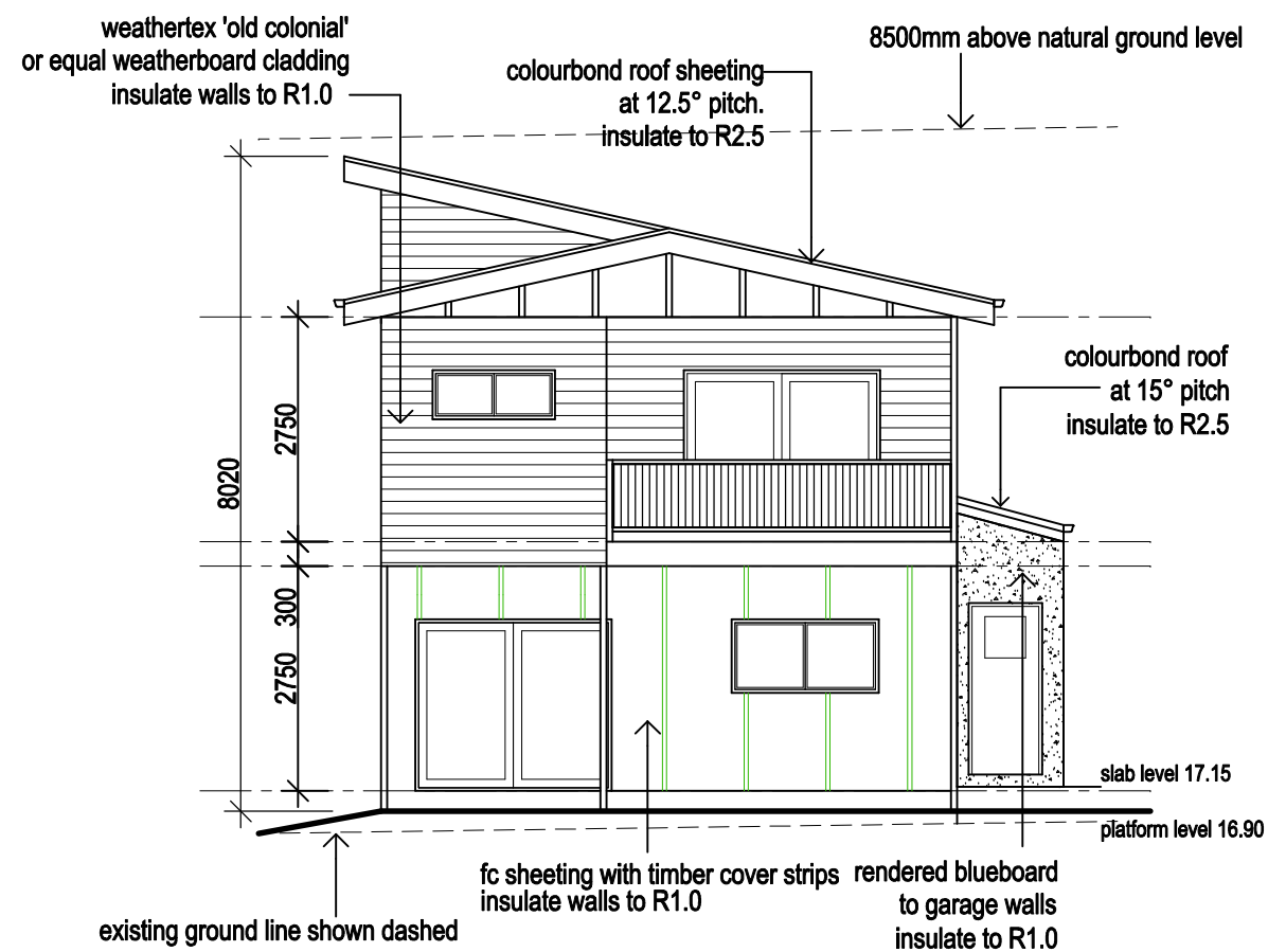
REAR ELEVATION
