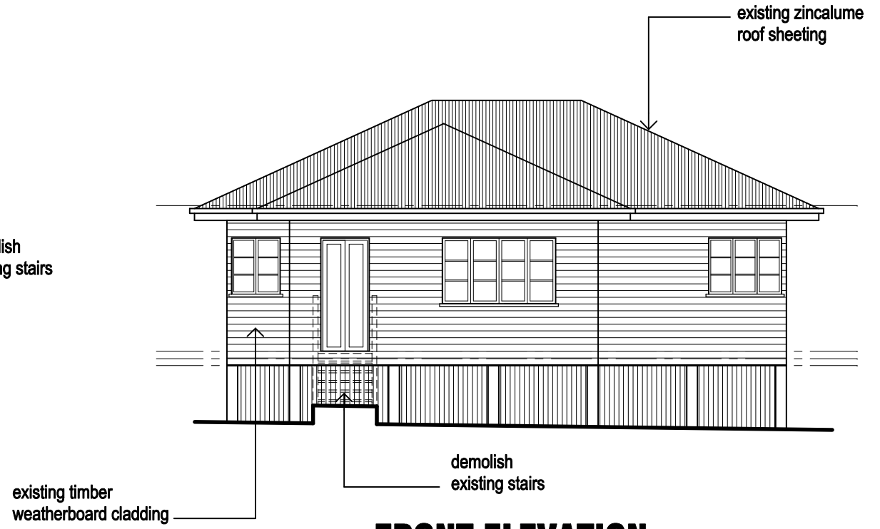
FRONT ELEVATION
