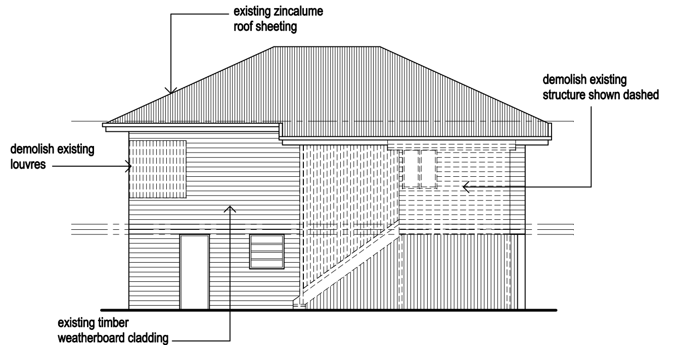
REAR ELEVATION
