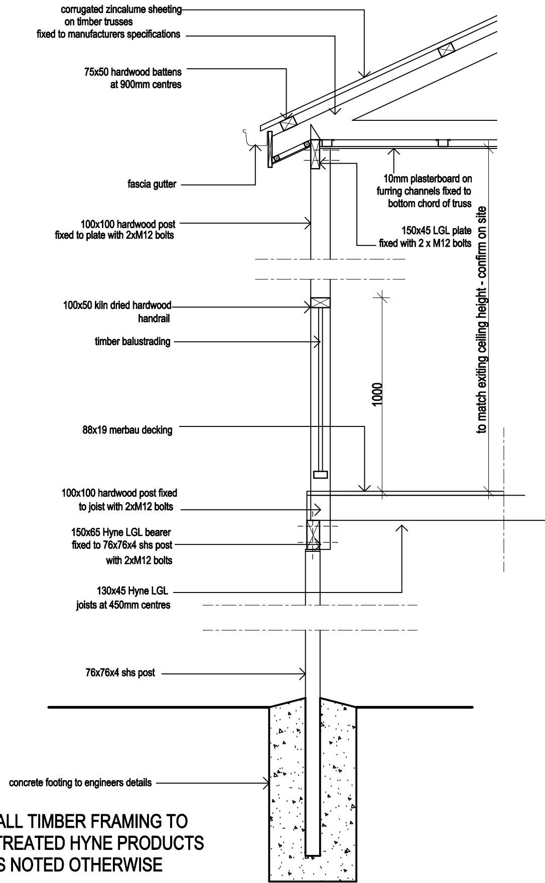
DECK SECTION 1 SCALE 1:20
