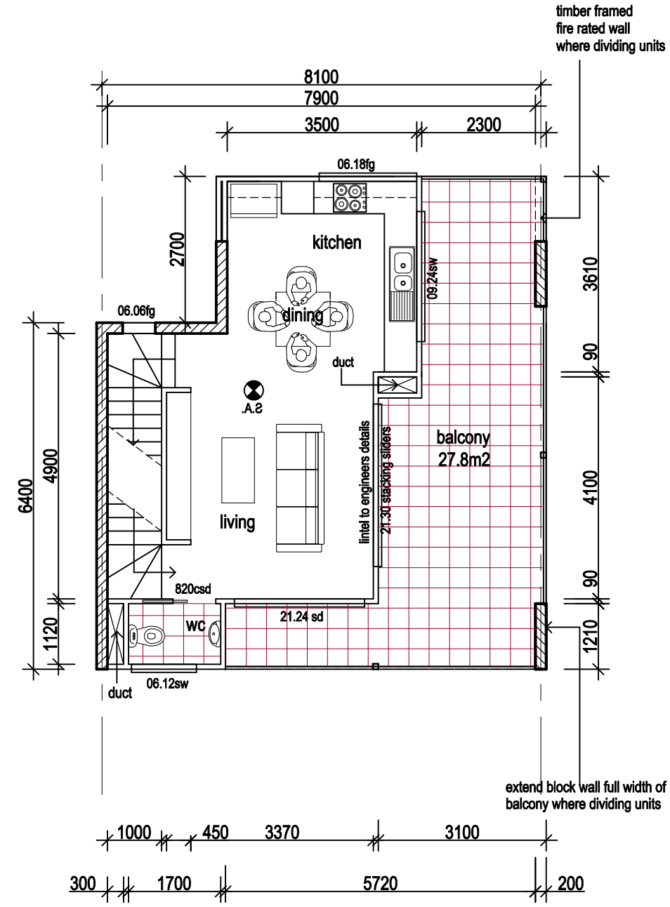
FIRST FLOOR gfa = 36.99
