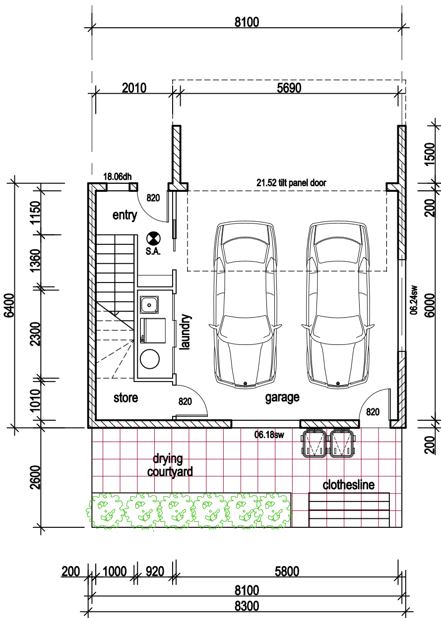
GROUND FLOOR gfa = 8.85m 2
