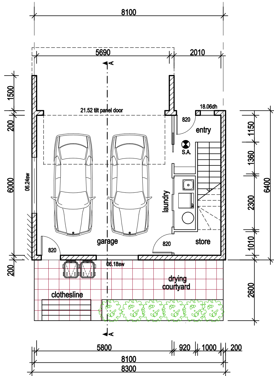
GROUND FLOOR gfa = 8.76m 2
