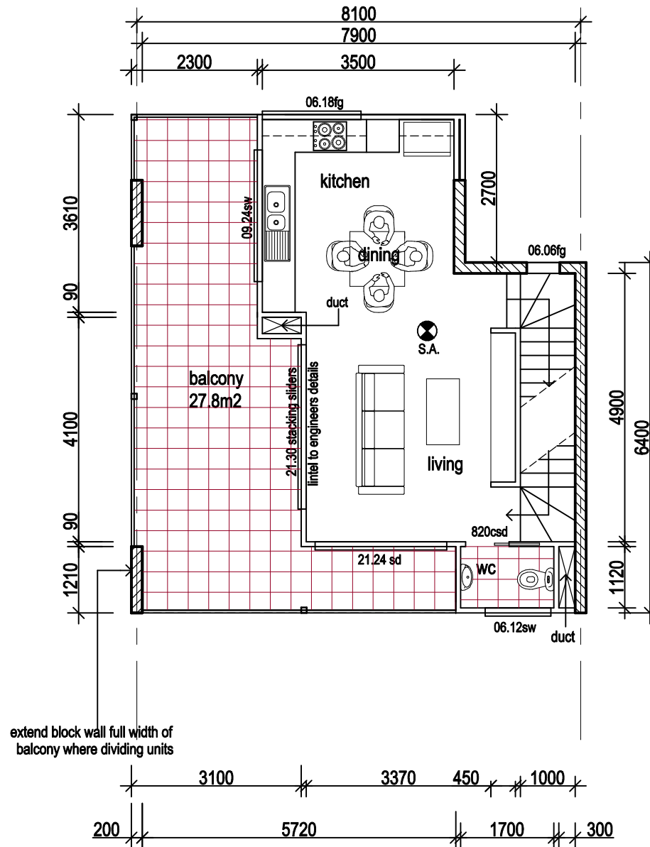
FIRST FLOOR gfa = 36.99
