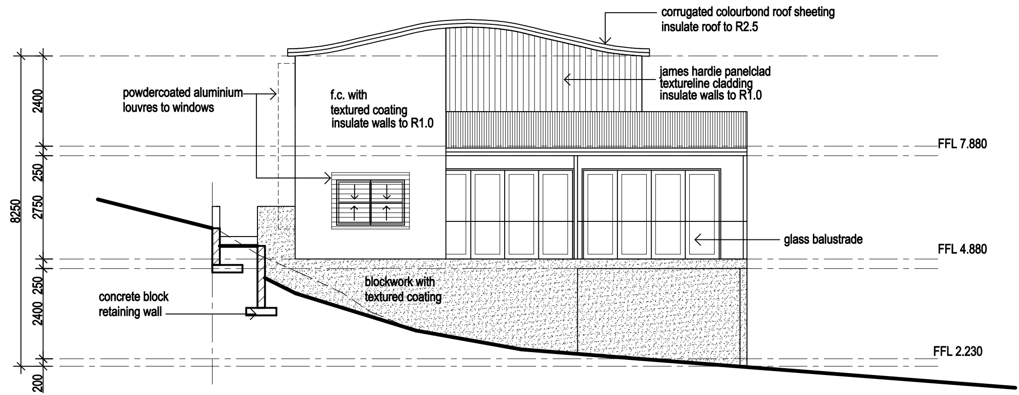
REAR ELEVATION
